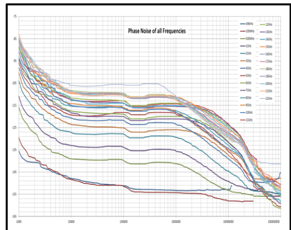
Phase Noise of all Frequencies
