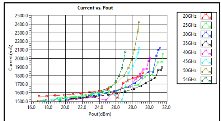
Current vs Output Power (+5VDC)
