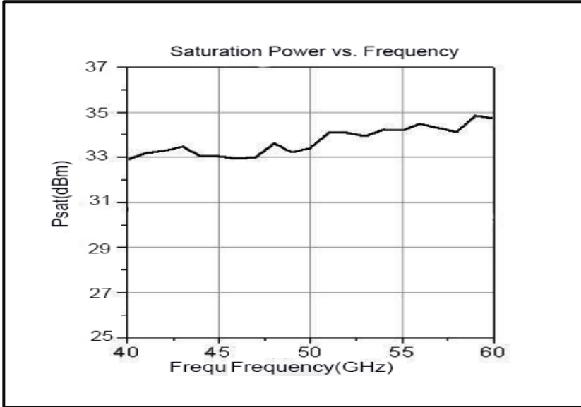
Saturation Power vs. Frequency
