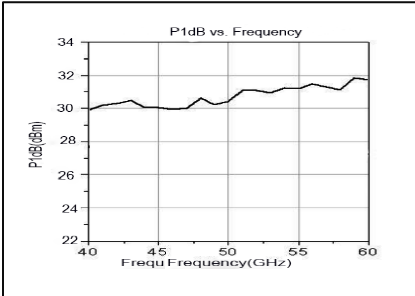
P1dB vs. Frequency
