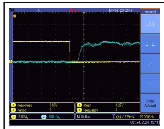
The Drains-Enable Rise Time is 25 us @+25°C
