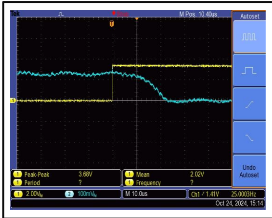
The Gates-Enable Fall Time is 20 us @+25°C
