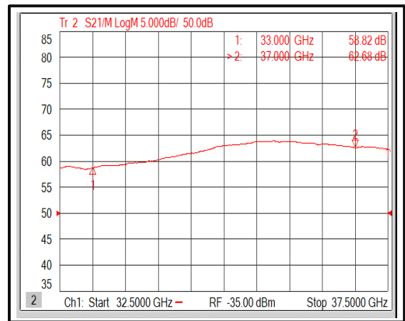
Gain @ -40°C
