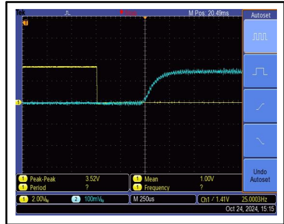
The Gates-Rise Time is 750 us @+25°C
