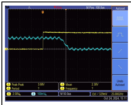
The Drains-Disable Fall Time is 100 us @+25°C
