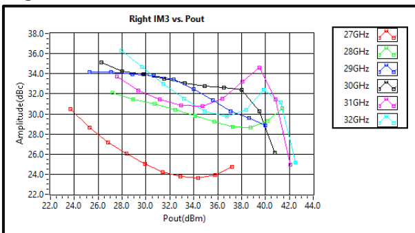
Right IM3 vs. Pout
