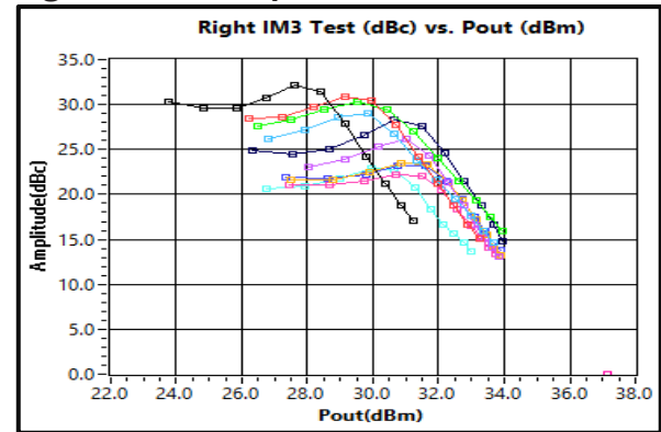
Right IM3 vs. Output Power 20GHz – 40GHz
