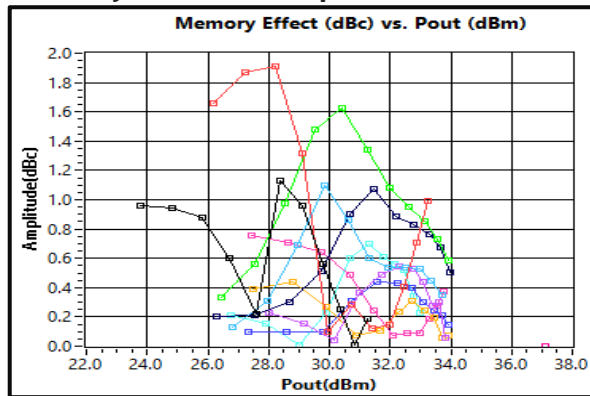
Memory Effect vs. Output Power 20GHz – 40GHz
