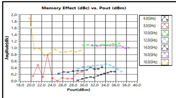
Memory Effect vs. Output Power 6GHz-18GHz
