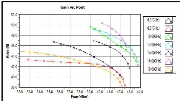
Gain vs. Output Power 6GHz-18GHz
