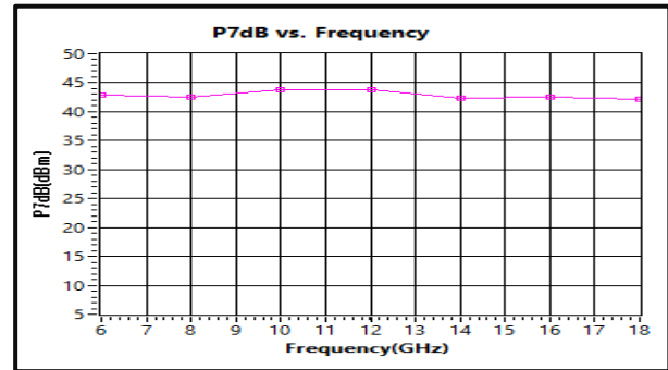
P7dB vs. Frequency 6GHz-18GHz
