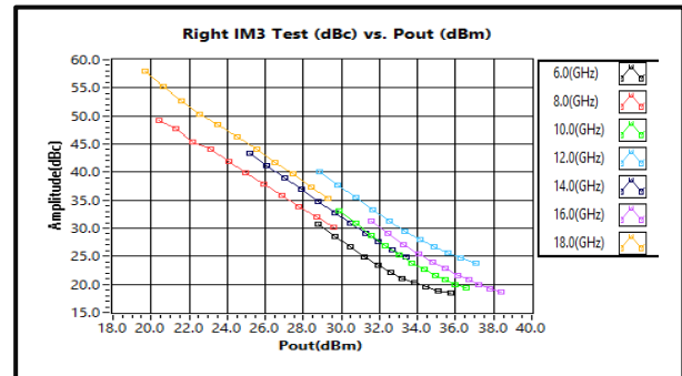
Right IM3 vs. Output Power 6GHz-18GHz
