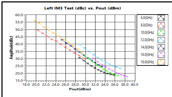
Left IM3 vs. Output Power 6GHz-18GHz
