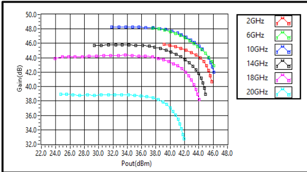
Psat vs Gain
