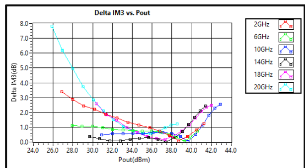
Delta IM3 vs. Output Power
