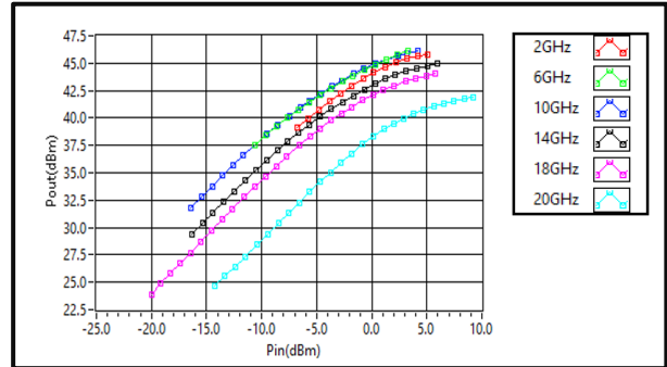
Pout vs Pin
