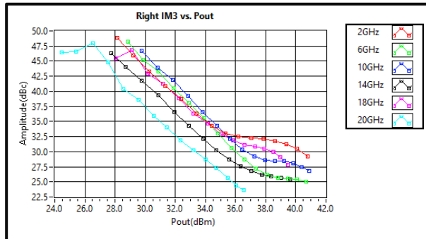
Right IM3 vs. Output Power
