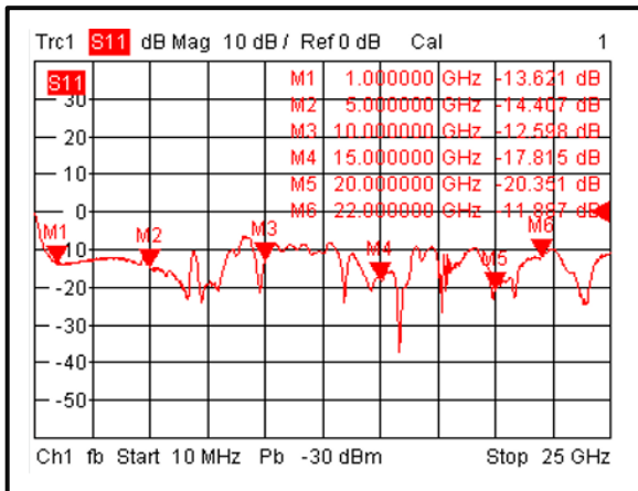
Input Return Loss @-40°C
