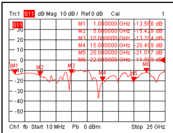
Input Return Loss @+85°C
