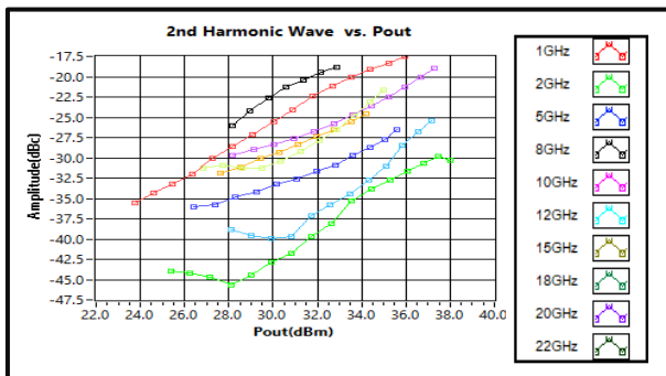
2nd Harmonic Wave vs Output Power
