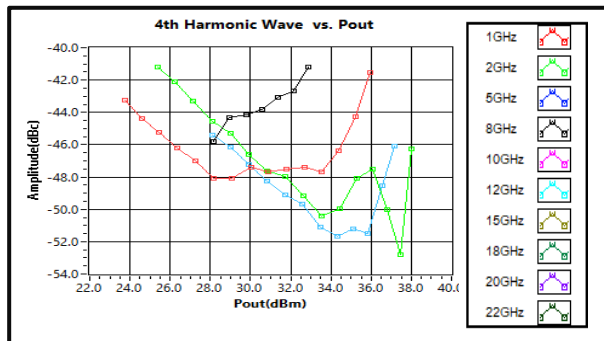
4th Harmonic Wave vs Output Power
