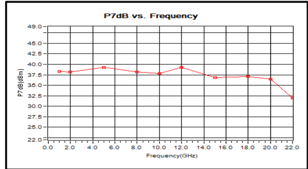
Saturated Power vs Frequency
