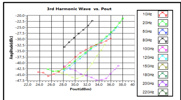
3rd Harmonic Wave vs Output Power
