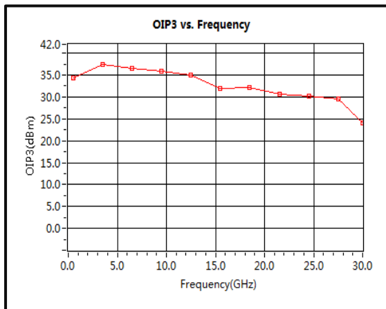
OIP3 vs. Frequency (CW Power)
