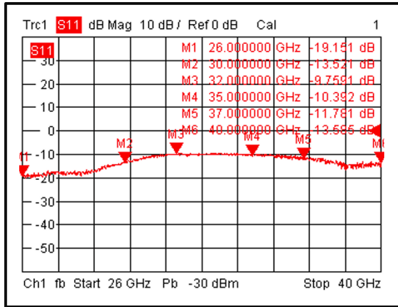
Input Return Loss vs Frequency @+85°C
