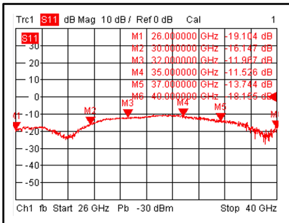
Input Return Loss vs Frequency @-40°C
