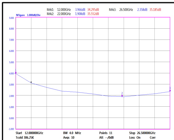
Noise Figure(12-26.5GHz)
