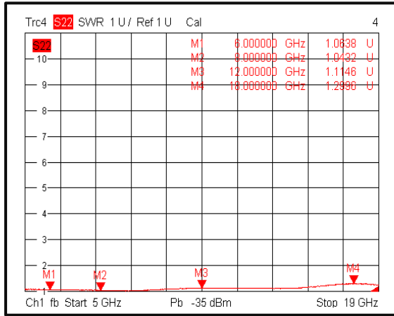
Output VSWR@+25°C
