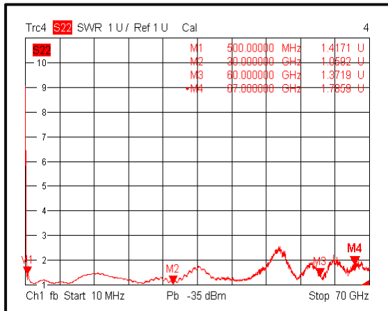
Output VSWR(0.5-67GHz)@+25°C
