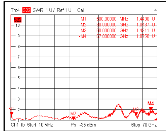
Output VSWR(0.5-67GHz)@+85°C
