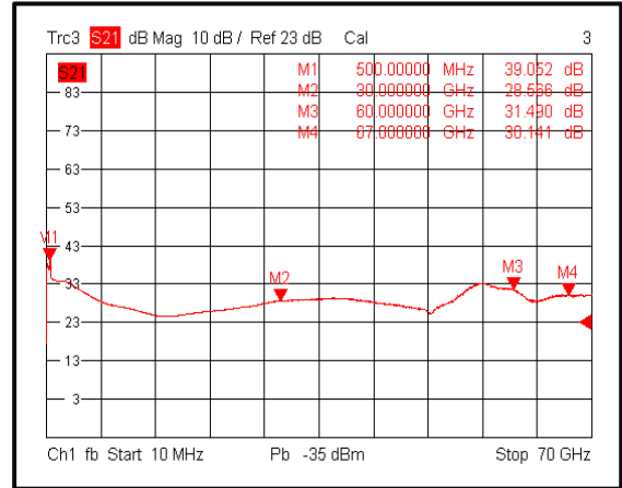
Gain(0.5-67GHz)@-40°C
