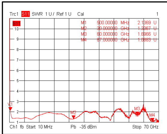
Input VSWR(0.5-67GHz)@+25°C
