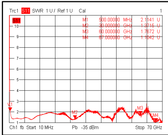
Input VSWR(0.5-67GHz)@+85°C
