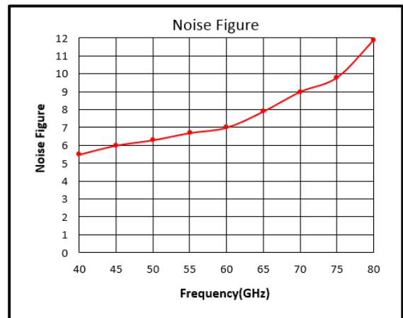
Noise Figure (40GHz-80GHz)
