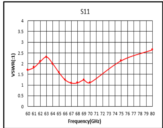
Input VSWR(60-80GHz)@+25°C
