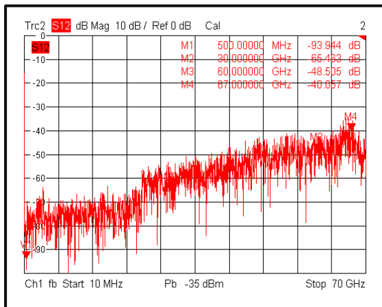
Isolation(0.5-67GHz)@-40°C
