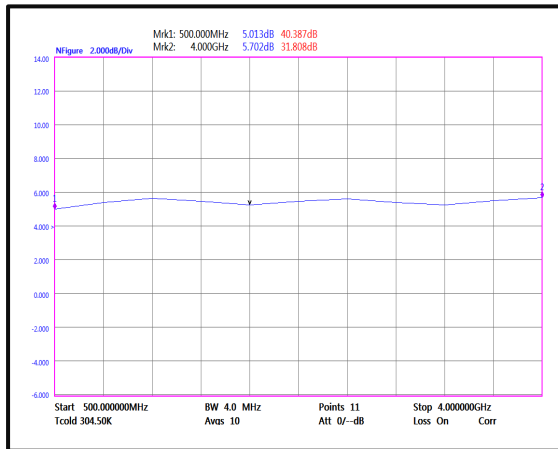
Noise Figure (0.5GHz-4GHz)
