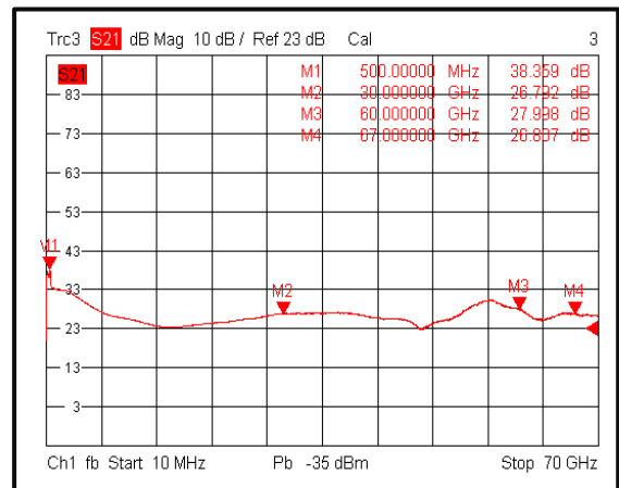
Gain(0.5-67GHz)@+85°C
