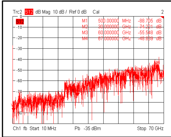
Isolation(0.5-67GHz)@+25°C
