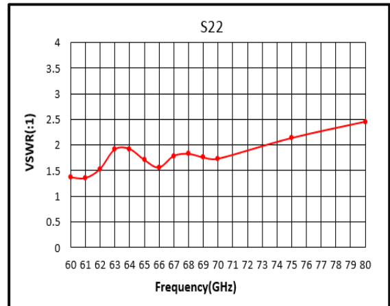
Output VSWR(60-80GHz)@+25°C
