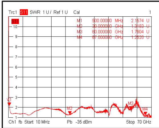
Input VSWR(0.5-67GHz)@-40°C
