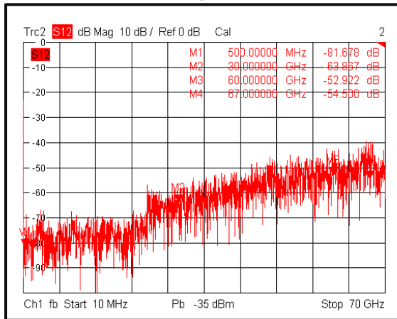
Isolation(0.5-67GHz)@+85°C
