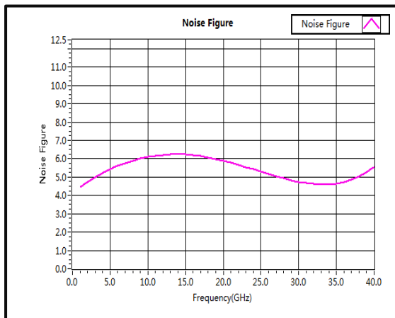
Noise Figure (0.5GHz-40GHz)
