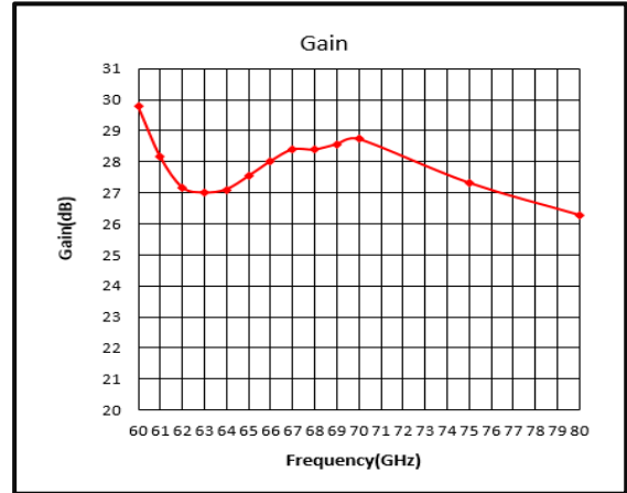
Gain(60-80GHz) @+25°C
