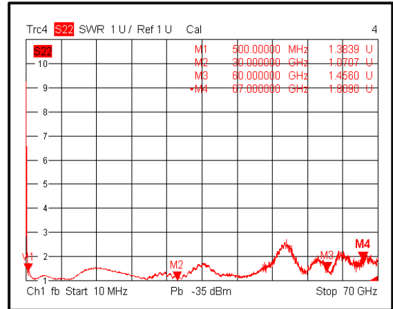
Output VSWR(0.5-67GHz)@-40°C
