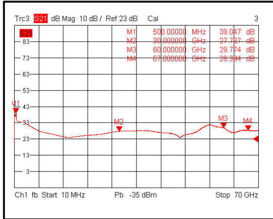
Gain(0.5-67GHz)@+25°C
