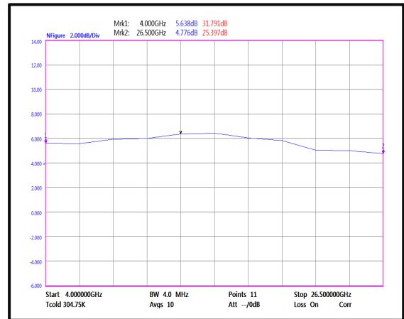
Noise Figure (4GHz-26.5GHz)
