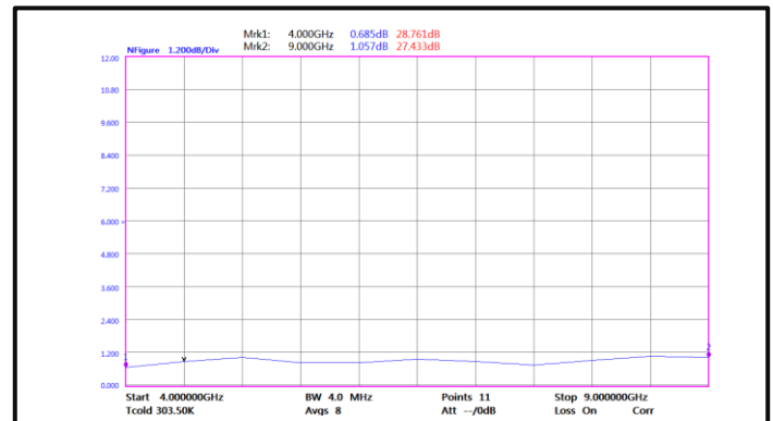
Noise Figure(4GHz-9GHz)
