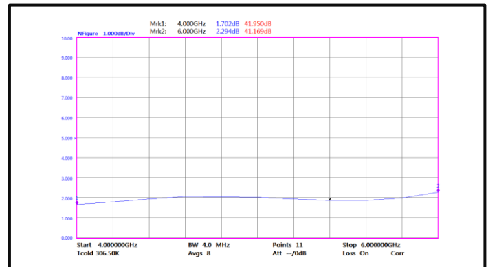
Noise Figure(4-6GHz)
