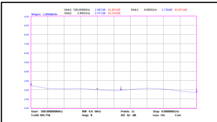
Noise Figure(0.5-4GHz)
