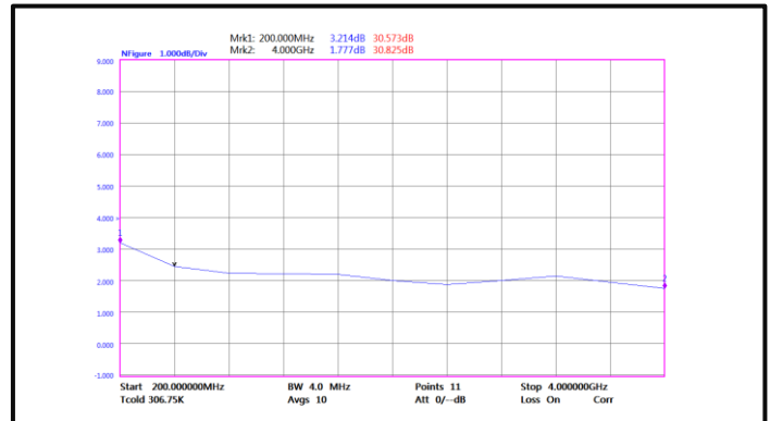
Noise Figure(200MHz-4GHz)
