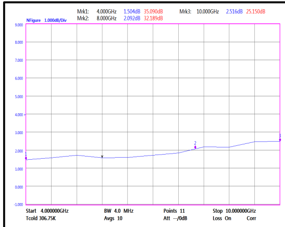
Noise Figure(4GHz-10GHz)
