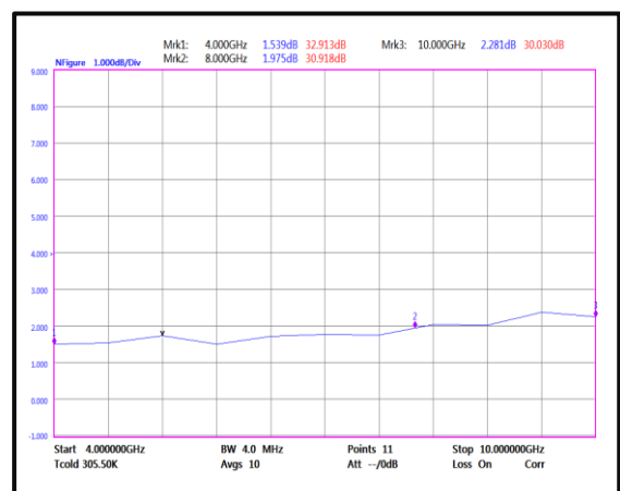
Noise Figure(4-10GHz)
