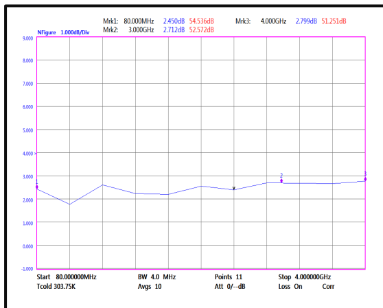
Noise Figure (80MHz-4GHz)
