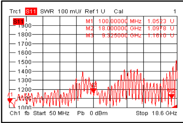
Primary VSWR (0.2-18GHz)
