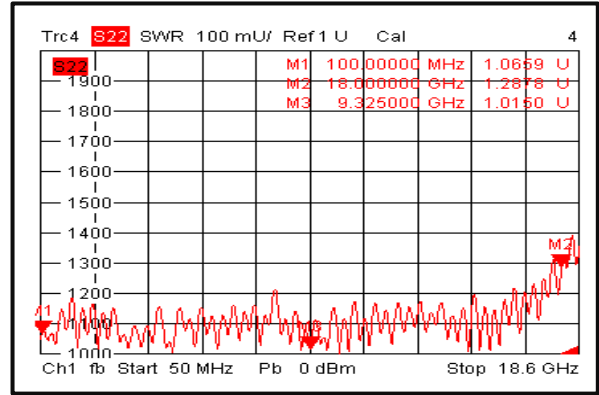
Secondary VSWR (0.2-18GHz)
