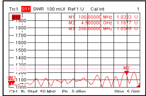
Primary VSWR (0.1-4.5GHz)
