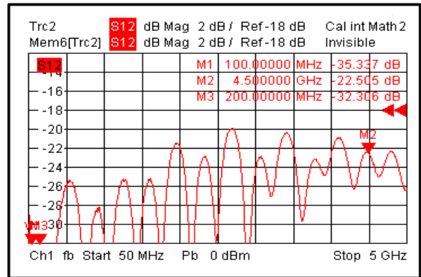
Directivity (0.1-4.5GHz)
