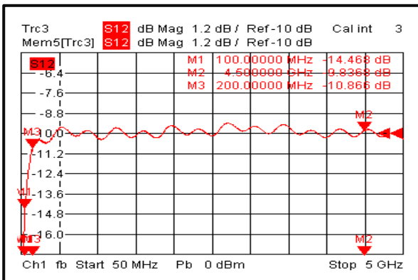
Nominal Coupling (0.1-4.5GHz)
