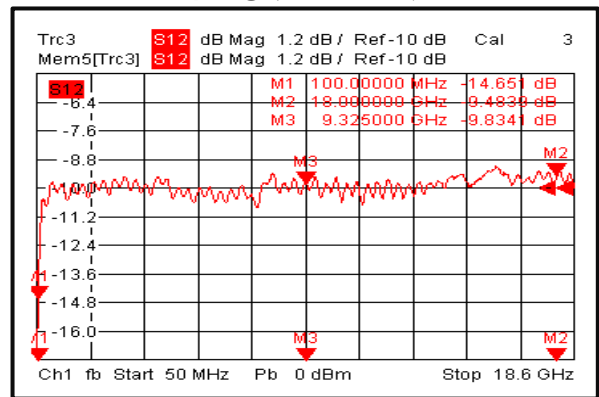
Nominal Coupling (0.2-18GHz)
