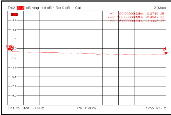
Insertion Loss (0.1-6GHz)
