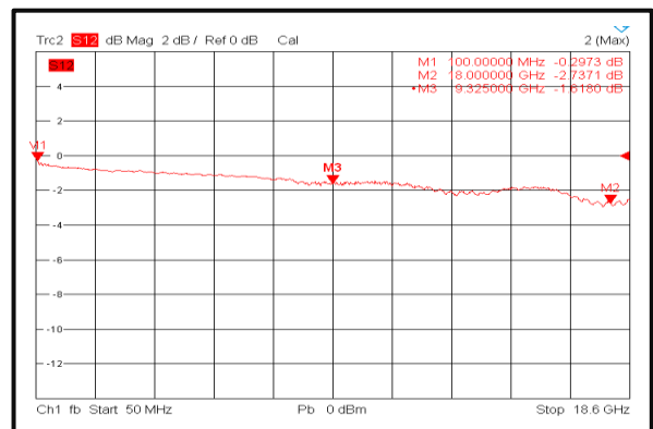
Insertion Loss (0.2-18GHz)
