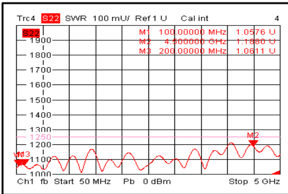
Secondary VSWR (0.1-4.5GHz)
