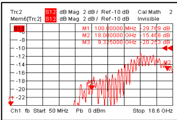
Directivity (0.2-18GHz)
