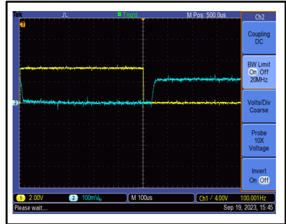
The Gate-Enable Fall Time is 50us ns @+25°C
