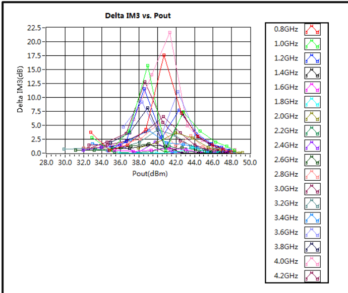
Delta IM3 vs. Pout
