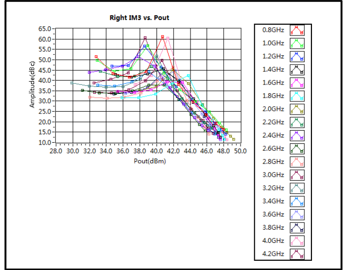
Right IM3 vs. Pout
