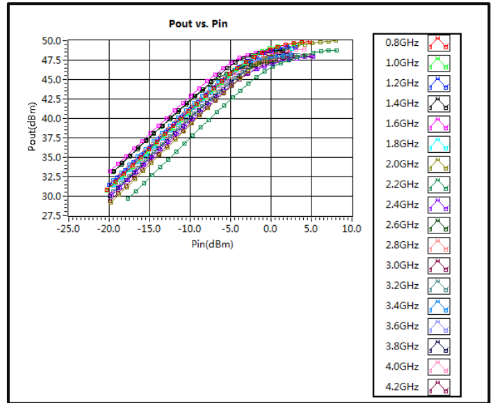
Pout vs. Pin
