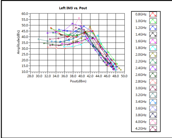
Left IM3 vs. Pout
