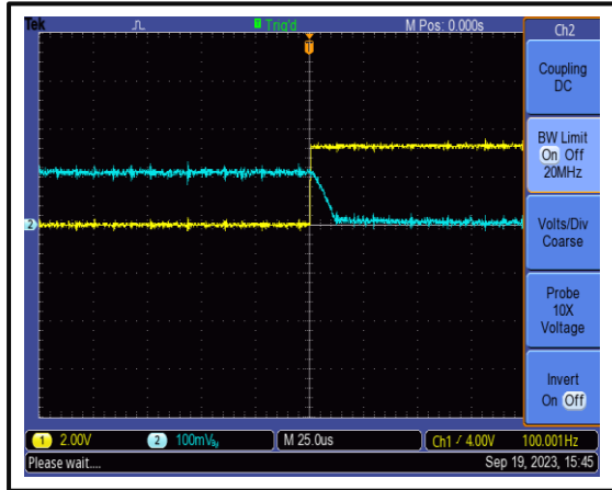
The Gate-Enable Rise Time is 20 us @+25°C
