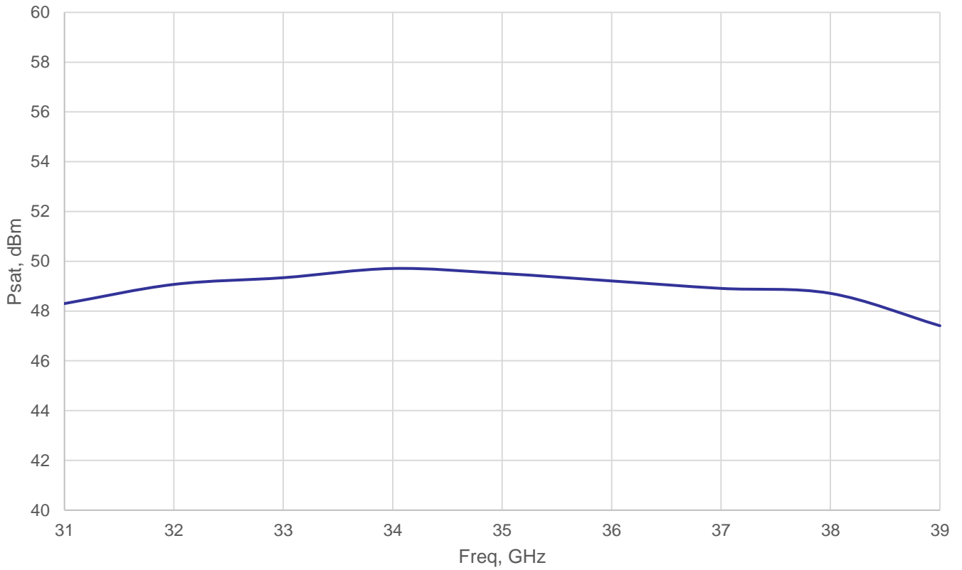
REMC32G38GF Psat vs. Freq
