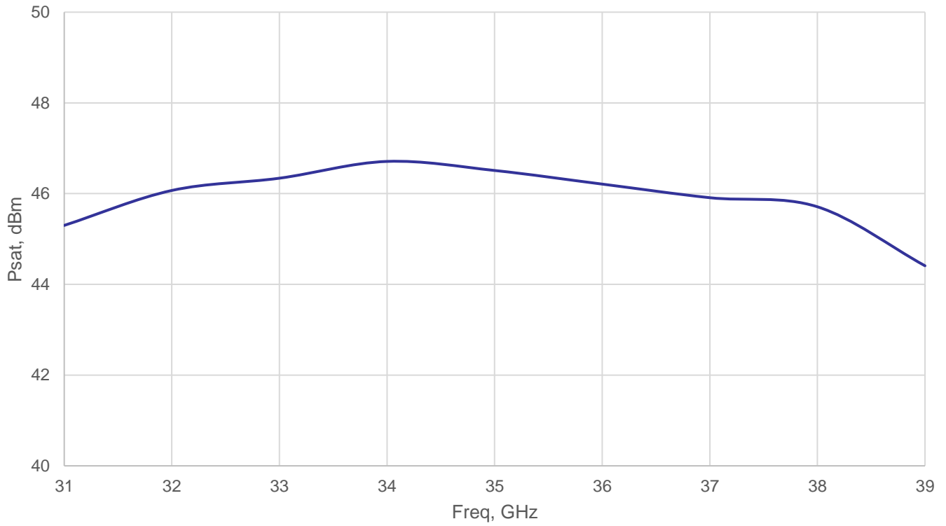
REMC32G38GE Psat vs. Freq
