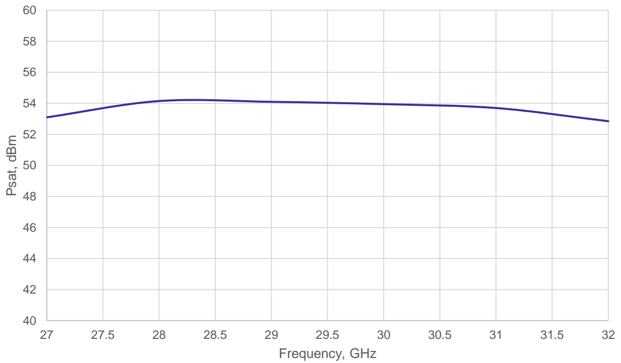
REMC27G31GF Psat vs. Freq
