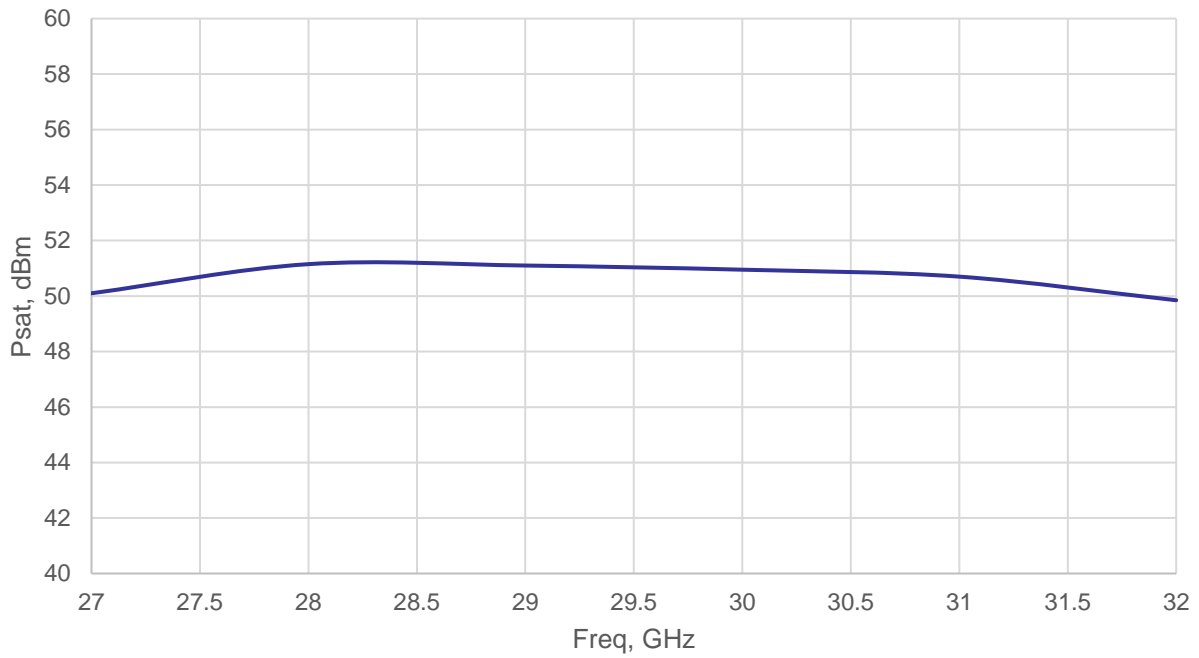
REMC27G31GE Psat vs. Freq
