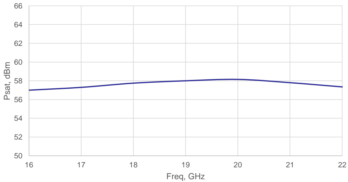
Psat vs. Freq
