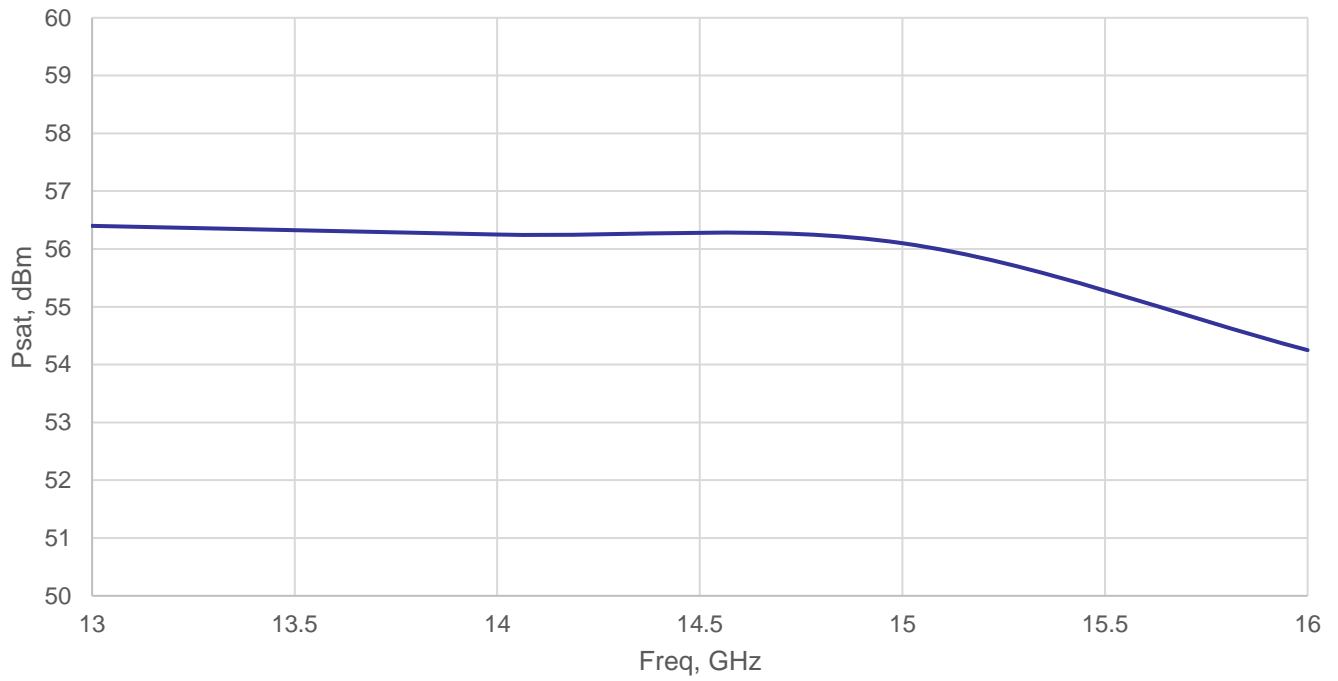
REMC13G16GE Psat vs. Freq
