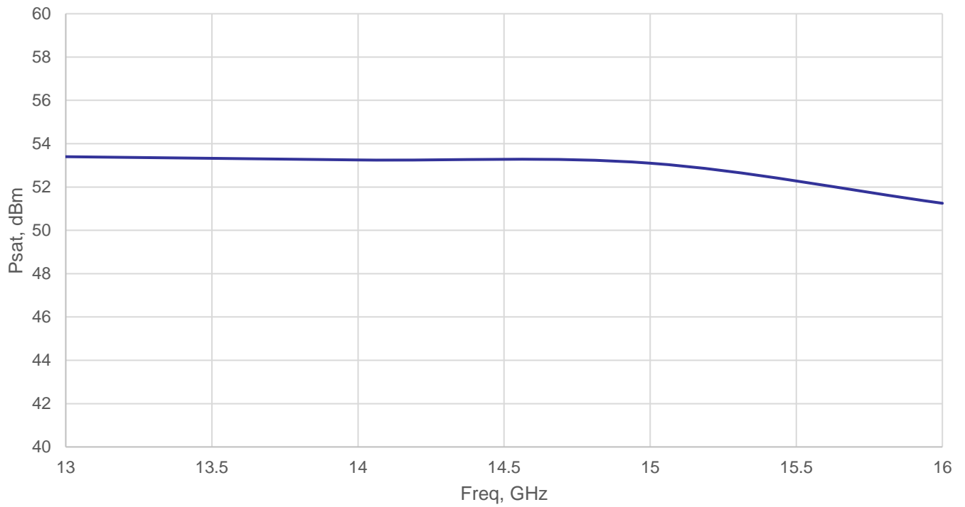
REMC13G16GD Psat vs. Freq
