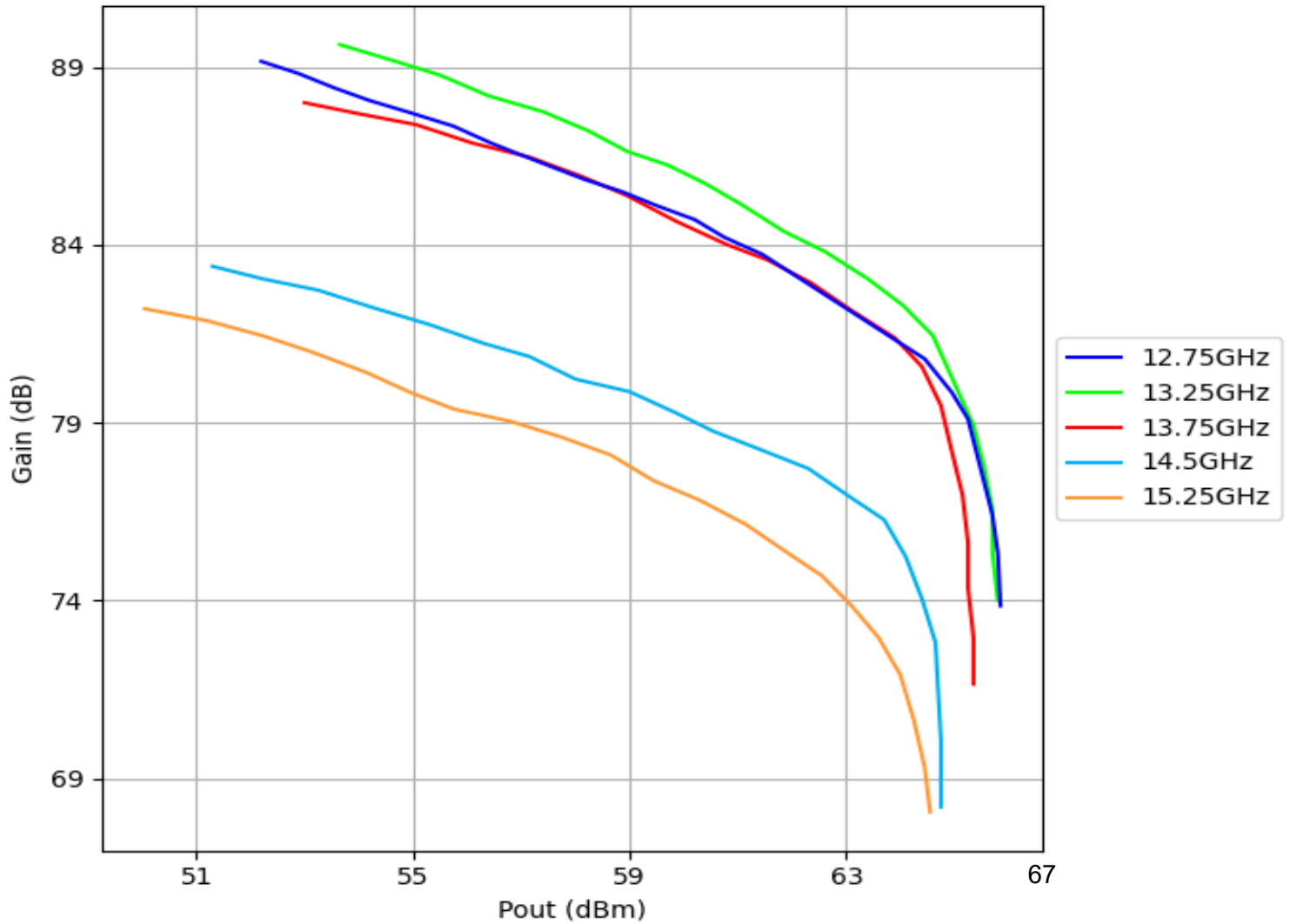
Gain vs. Pout
