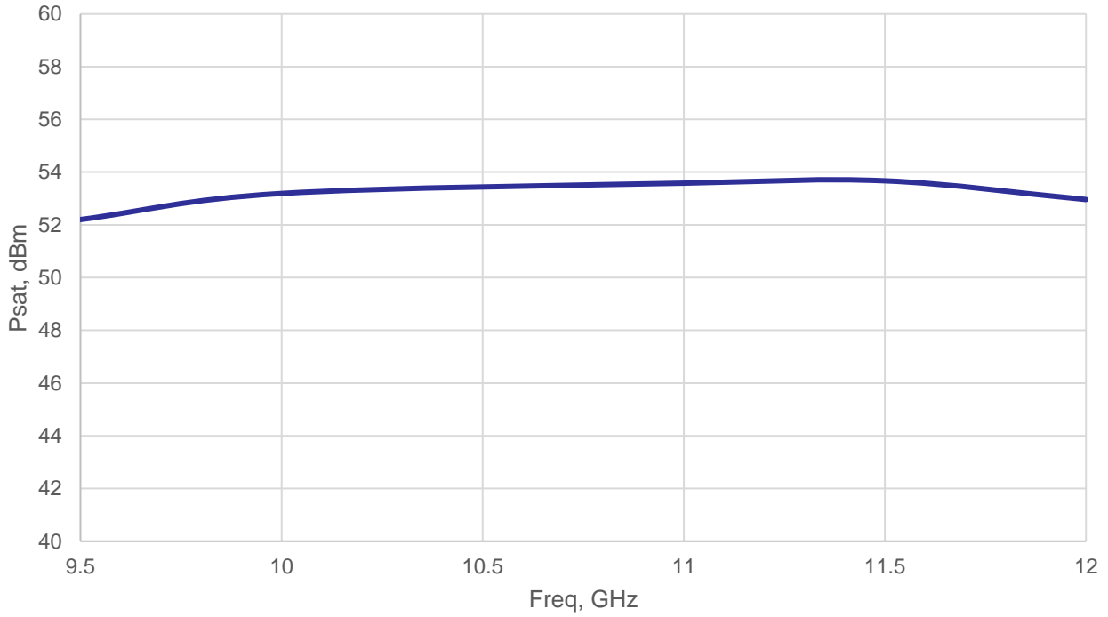
REMC10G11GF Psat vs. Freq
