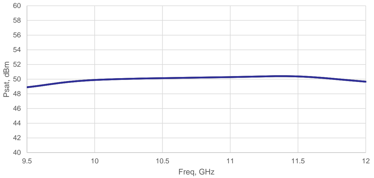
REMC10G11GD Psat vs. Freq
