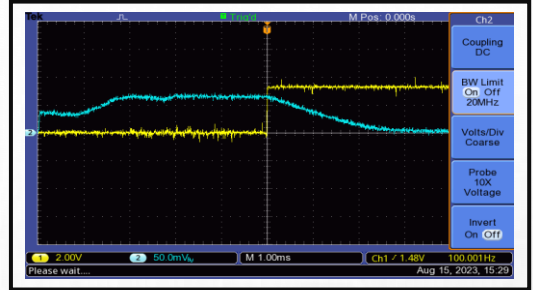
The Drains Closure Time is 3000 us
