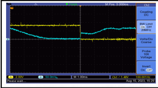
The Drains Open Time is 3000 us
