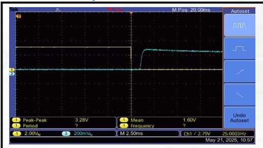
The Drains Open Time is 2000 us
