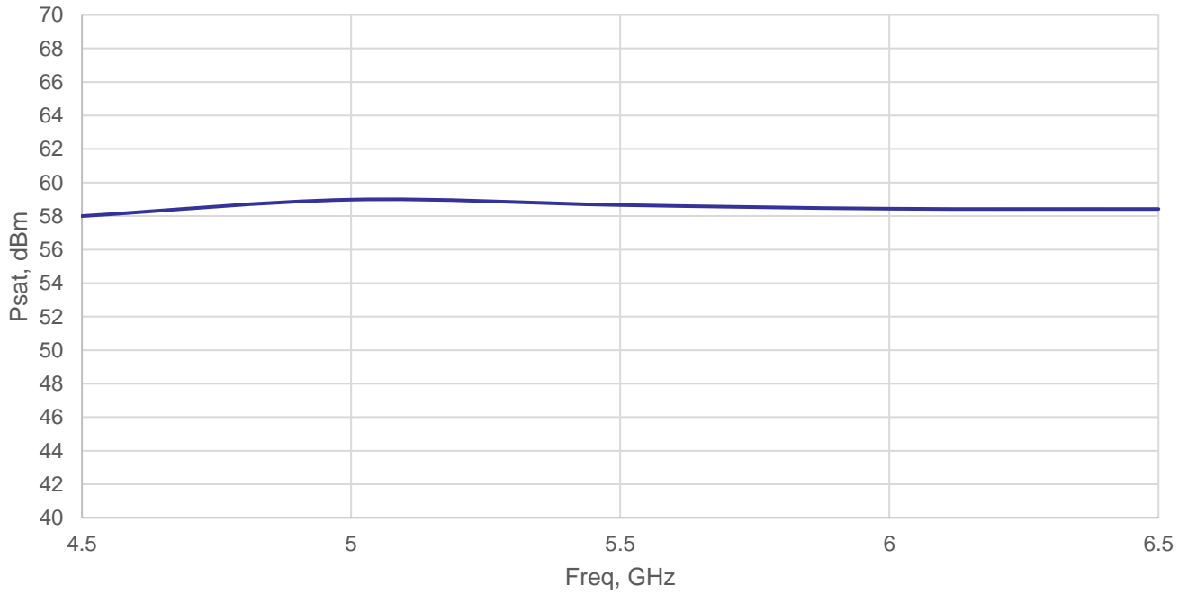
REMC0506GF Psat vs. Freq
