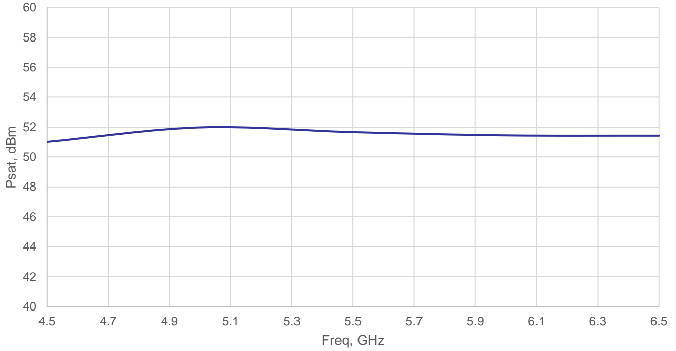
REMC0506GD Psat vs. Freq
