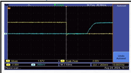
The Drains Open Time is 7 ms
