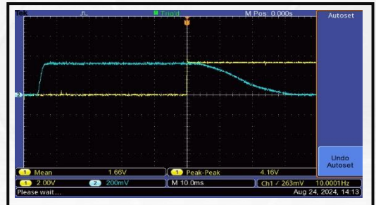
The Drains Closure Time is 30 ms
