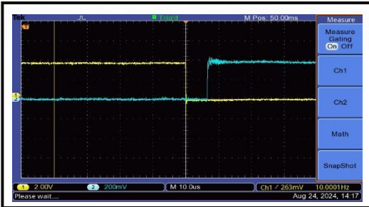
The RF Switch On Time is 8 us
