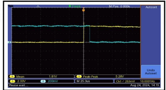
The RF Switch Off Time is 10 us
