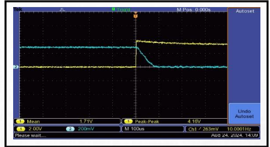
The Gates Closure Time is 100 us
