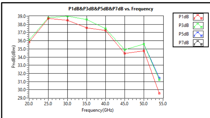
PxdB vs Frequency CW @ +25°C
