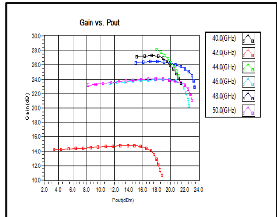
Gain vs. Pout (40 GHz to 50GHz)
