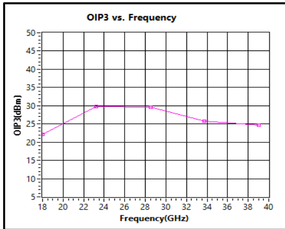
OIP3 vs. Frequency (18GHz to 40GHz)
