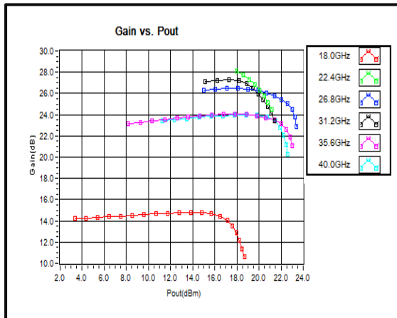
Gain vs. Pout (18GHz to 40GHz)
