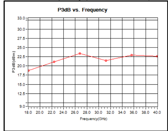
P3dB vs. Frequency (18GHz to 40GHz)
