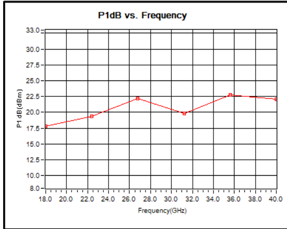
P1dB vs. Frequency (18GHz to 40GHz)
