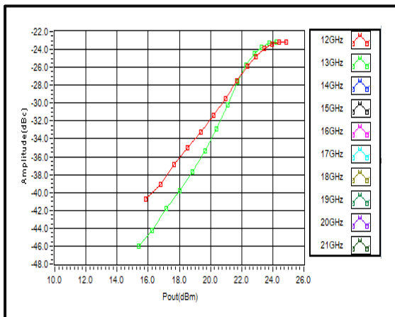
3rd Harmonic Wave vs. Pout
