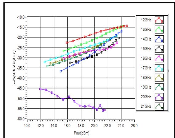
2nd Harmonic Wave vs. Pout
