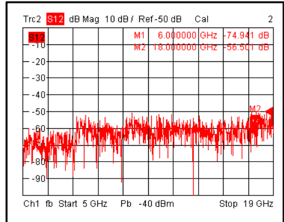
Isolation @+85°C
