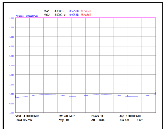
Noise Figure(4-8GHz)
