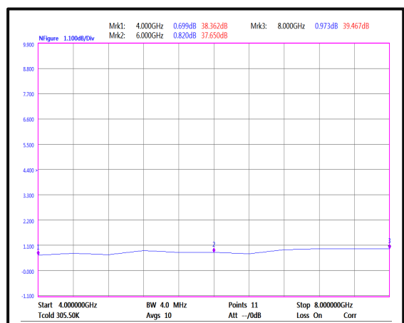
Noise Figure (4GHz-8GHz)
