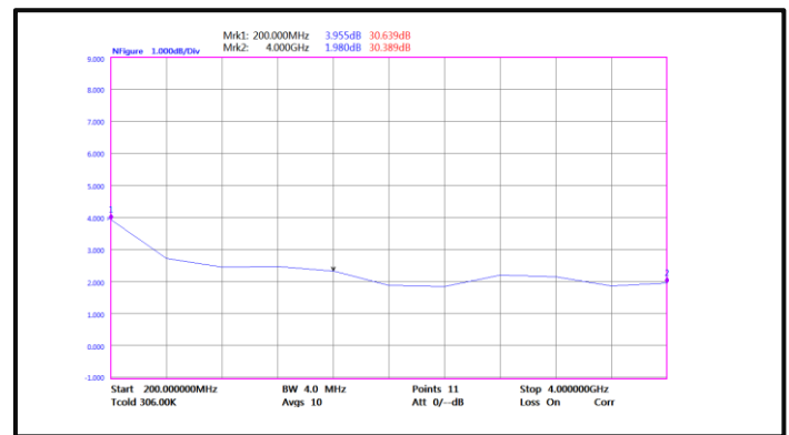
Noise Figure(0.2-4GHz)
