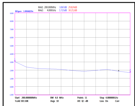
Noise Figure(0.2GHz-4GHz)
