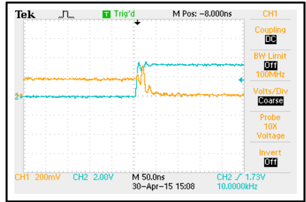
Switching Speed
