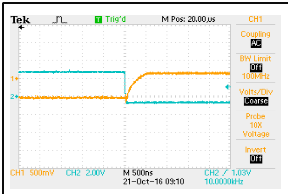
Rise time
