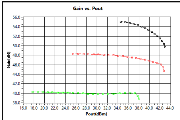
Gain vs. Output Power 32GHz-34GHz
