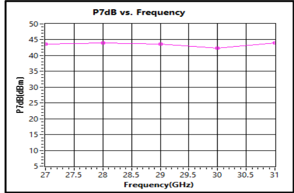
P7dB vs. Frequency 27GHz-31GHz
