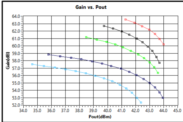
Gain vs. Output Power 27GHz-31GHz
